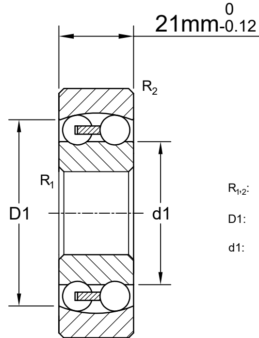
LILY BEARING
