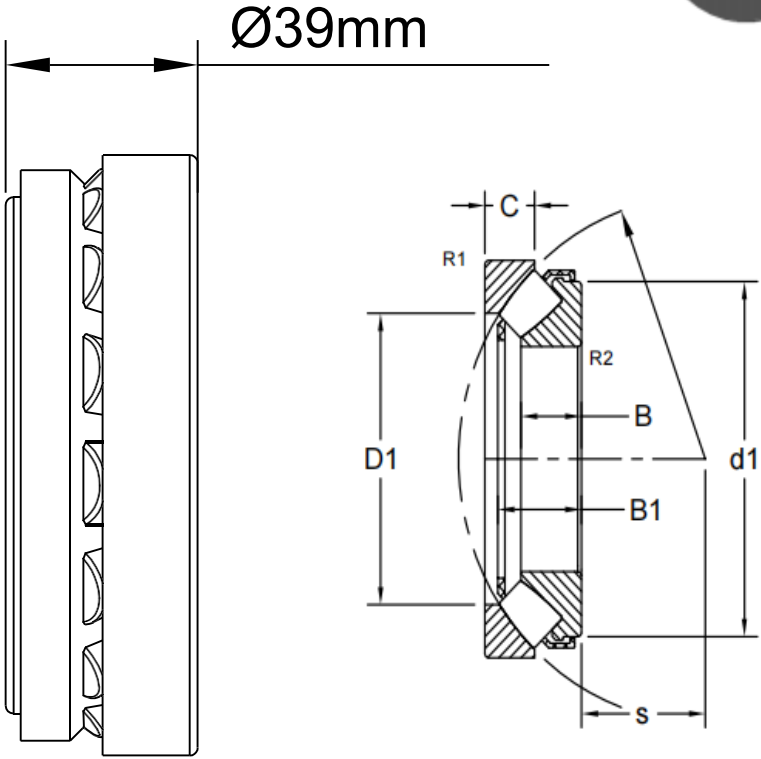
LILY BEARING
